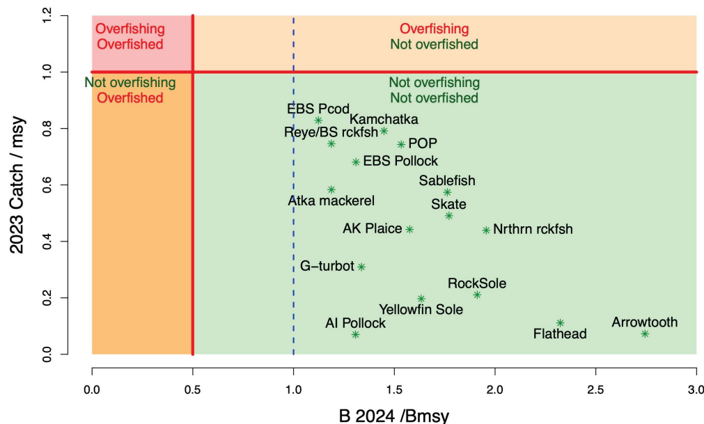
Figure 3 Summary of Bering Sea stock status next year (spawning biomass relative to BMSY; horizontal axis) and current year catch relative to fishing at FMSY (vertical axis) where FOFL is taken to equal FMSY. Source: Aydin et al., 2023.
