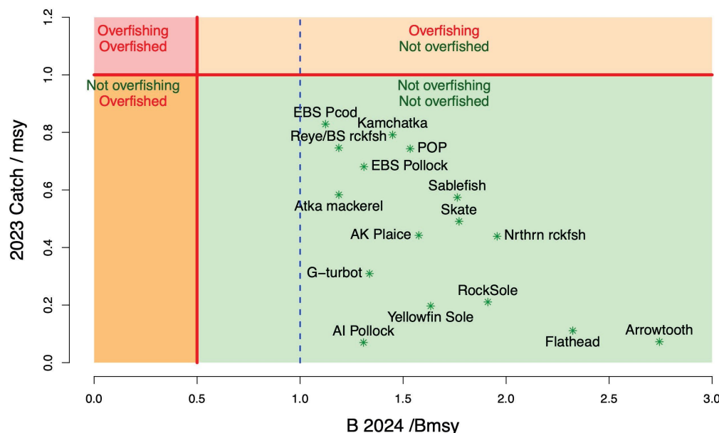
Figure 1 Summary of Bering Sea stock status next year (spawning biomass relative to BMSY; horizontal axis) and current year catch relative to fishing at FMSY (vertical axis) where FOFL is taken to equal FMSY. Source: Aydin et al., 2023.
